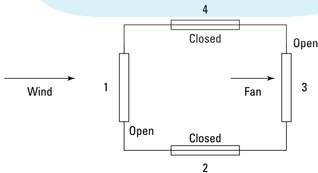
Figure 13-2: Locating fans to enhance the natural ventilation scheme.
